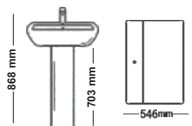
DUNA BP-2 Dimensions:
