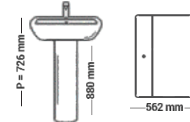
RAVI BP-1 Dimensions:
