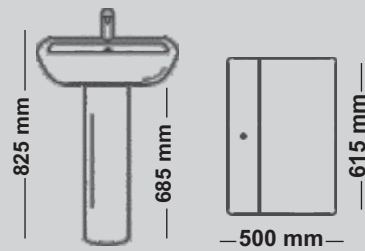
FANTASY BP-11 Dimensions:
