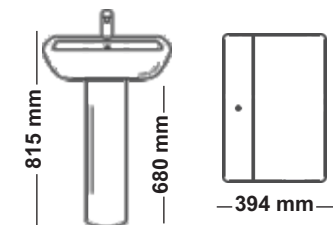
(SMALL) MEHRAN BP-14 Dimensions:
