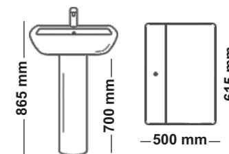
FLORA BP-15 Dimensions:
