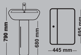
Casa BP-24 BASIN PEDESTAL
