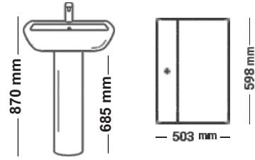
PEARL BP-16 Dimensions:
