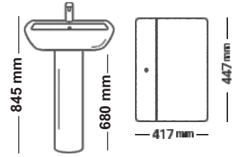
CLADA BP-17 Dimensions:
